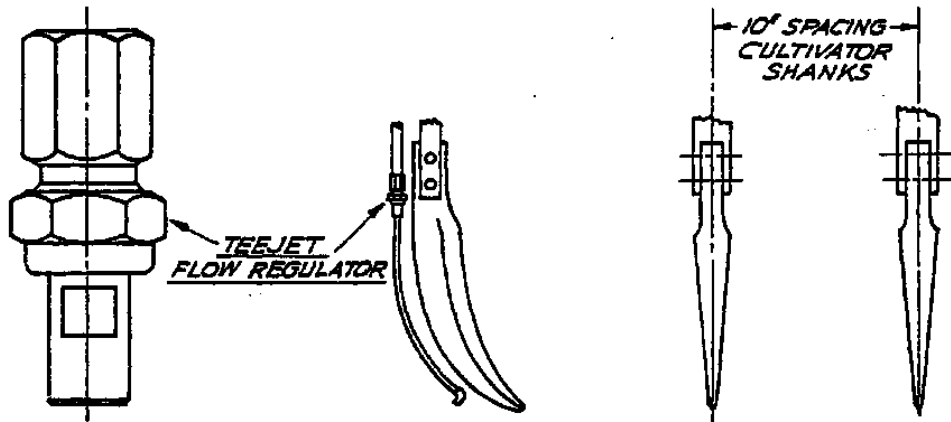
VIEWS SHOWING TYPICAL MOUNTING OF TEEJET FLOW REGULATOR & SHANK SPACING
