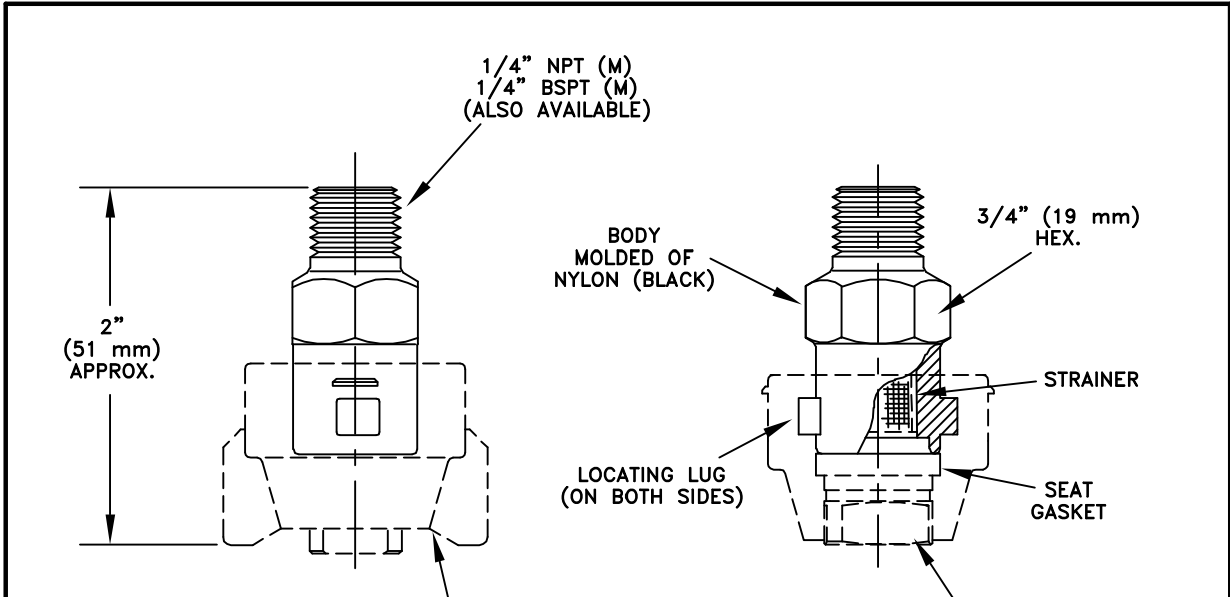
QUICK TEEJET® CAP WITH GROOVES THAT FIT LOCATING LUGS OF BODY – CELCON. YELLOW COLOR STANDARD. (OTHER COLORS OPTIONAL)
