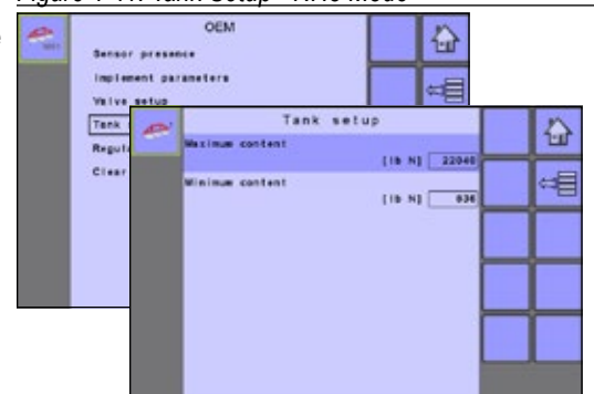
Figure 1-11: Tank Setup - NH3 Mode
