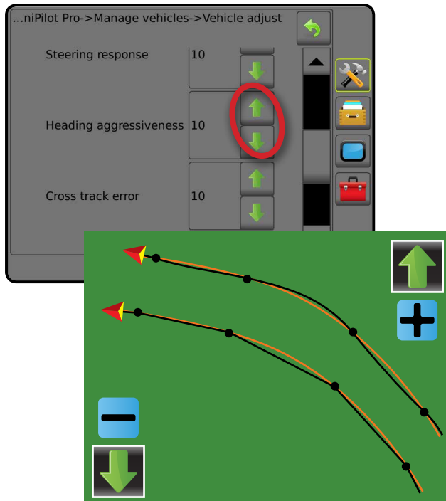
Figure 33: Heading aggressiveness
