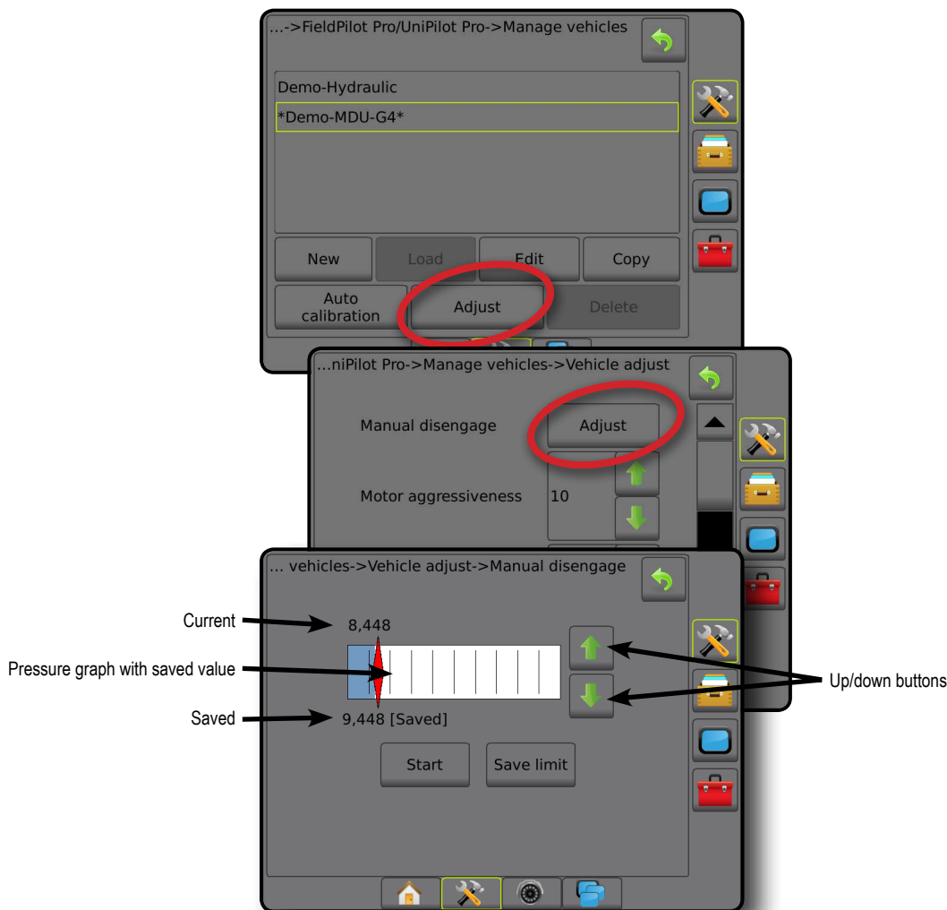
Figure 16: Manual disengage
