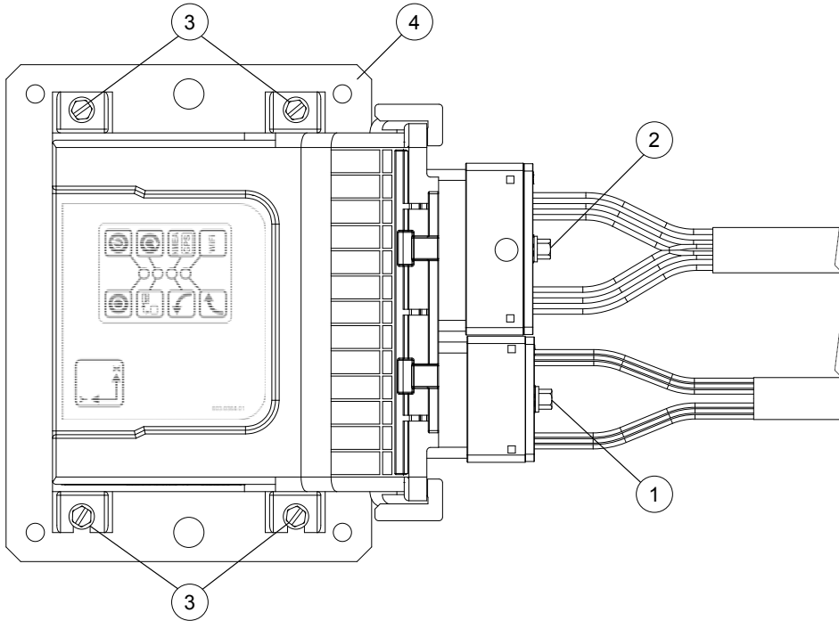
Figure 37: SCM Pro Installation Diagram
