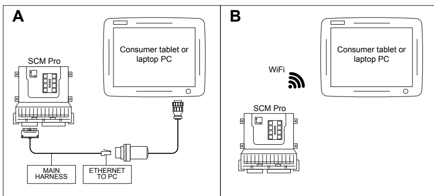
Figure 38: Display Connections
