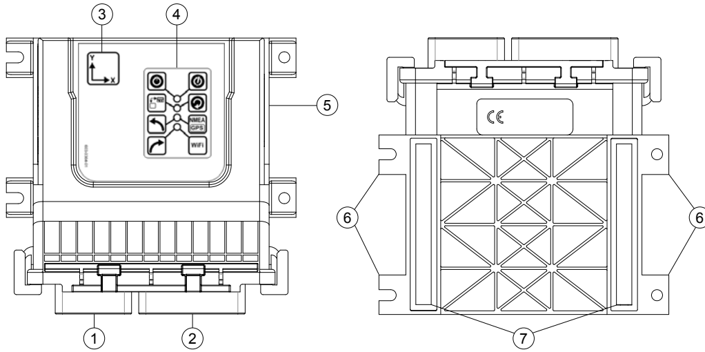
Figure 1: SCM Pro top and bottom views
