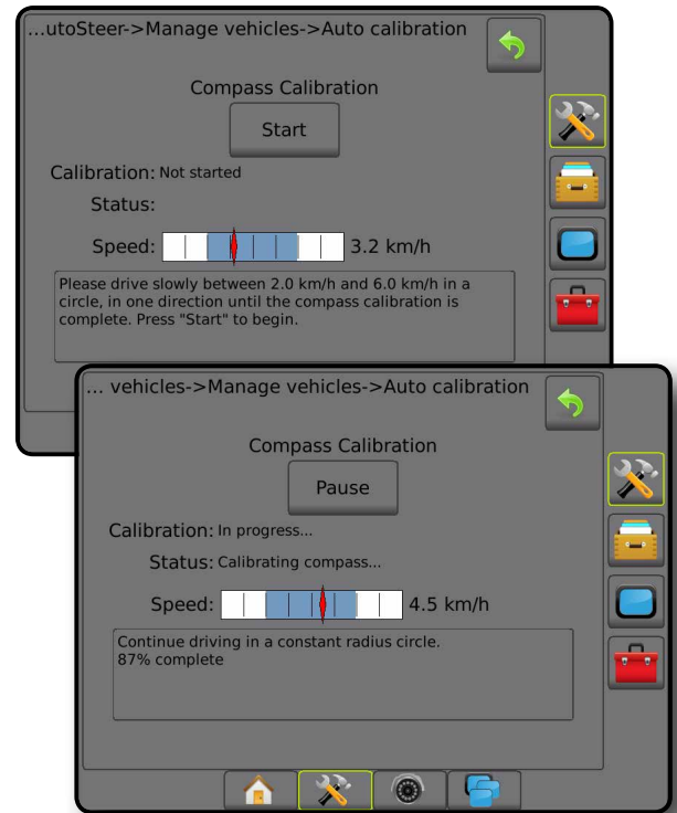
Figure 19: Compass calibration
