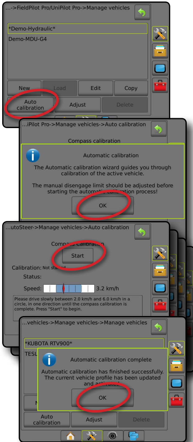
Figure 18: Automatic calibration
