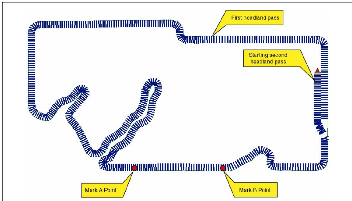
Figure 35: Starting the Second Headland Pass
