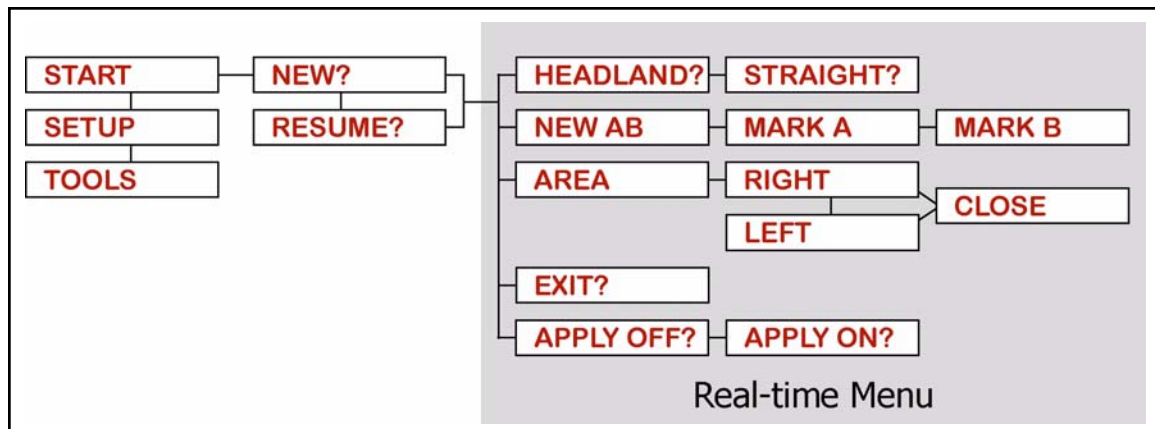
Figure 30: Real-Time Operation Flow Diagram
