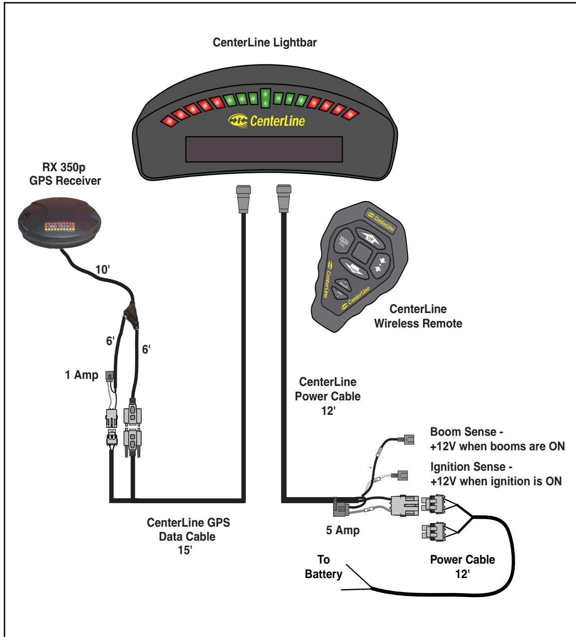
Figure 8: CenterLine with RX 350p WAAS DGPS Receiver
