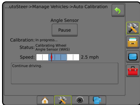
Figure 25: Angle Sensor Calibration in Progress
