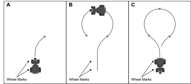
Figure 22: Driving Around for Tilt Calibration
