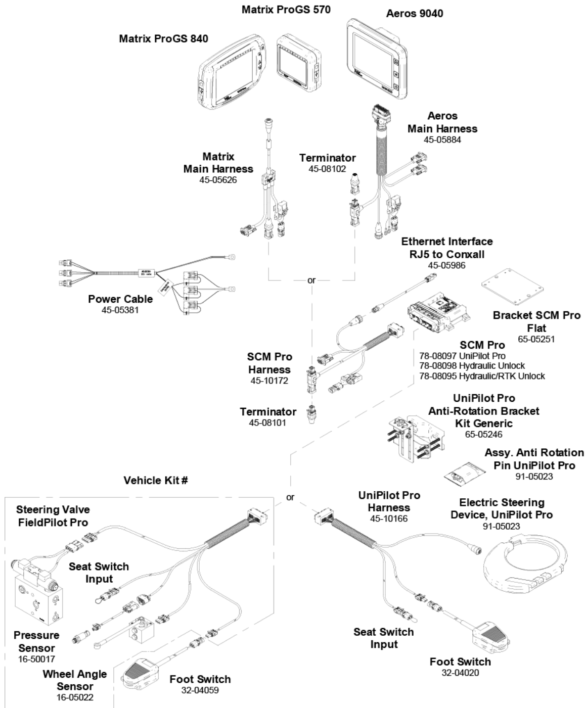
Figure 3: SCM Pro Connections
