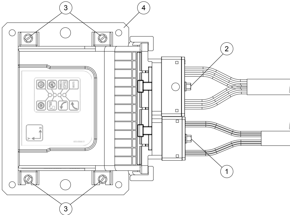
Figure 37: SCM Pro Installation Diagram
