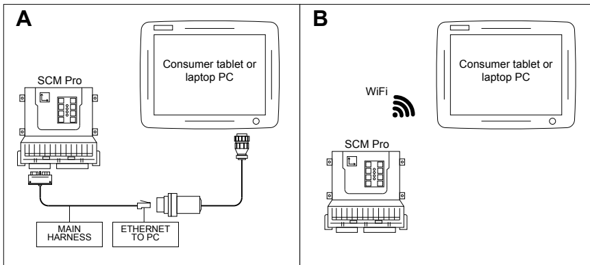
Figure 38: Display Connections
