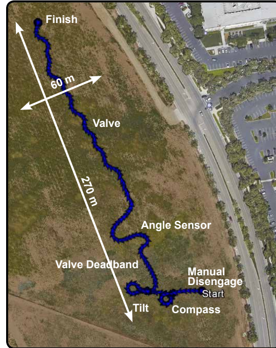
Figure 17: Calibration Trajectory Example
