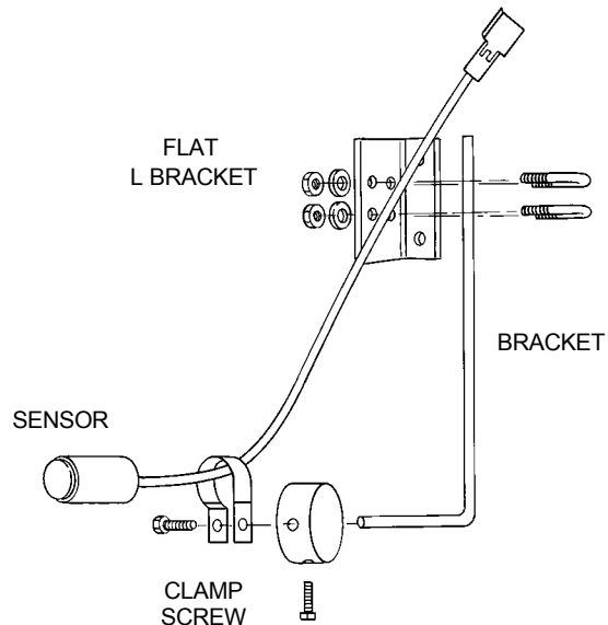
Figure 10: Sensor Assembly
