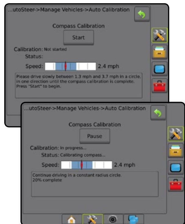
Figure 19: Compass Calibration
