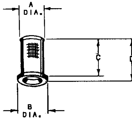
STRAINER ASSEMBLY
